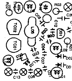
VCO UNIT
