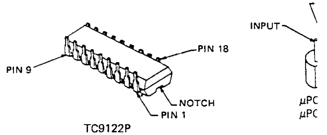
Viewed from component side
