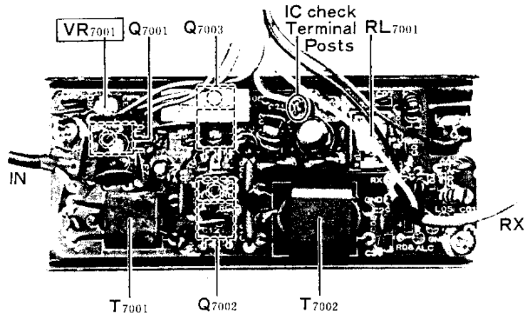
HF PA UNIT
